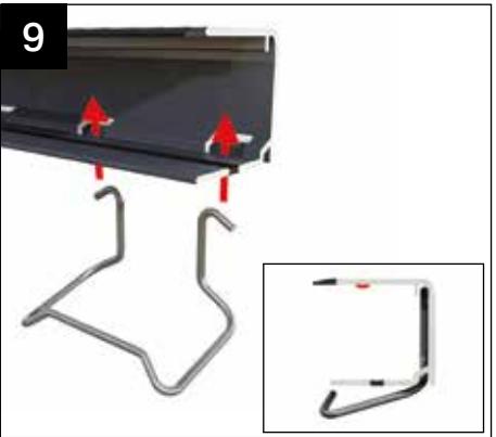
To retain the glazing to the valley wing, fit 2 wire clips (100mm from each end of the profile). The 'hooked ears' locate behind the lip detail as shown. Apply a continuous bead of sealant (MS Polymer to self cleaning glass). See Step 37 on page 16.
