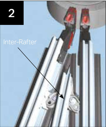
Bolt down using the nuts provided - ensure glazing platforms are level.
