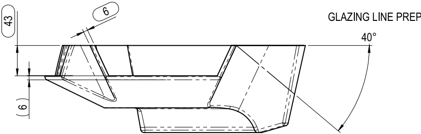
40° RIDGE PREP
